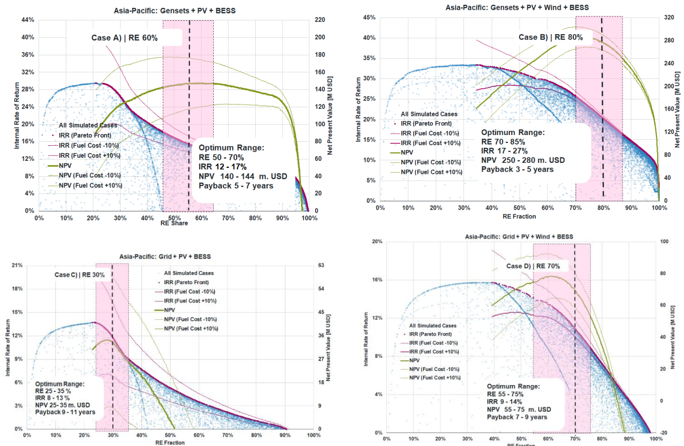
Figure 3 Illustration of the results from the hybrid simulations for off grid and grid connected hybrid systems
